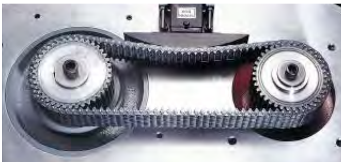
It is also possible to use sliding rails to tension the inverted tooth chains on the backside. The bending radius for HPC inverted tooth chains should be at least 30 times the pitch used. A factor of 20 is sufficient for all other types of inverted tooth chains.
